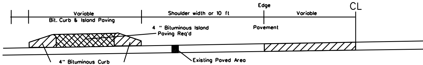
Typical Section of Bit. Curb & Bit. Island Placement on Existing Paved Areas
