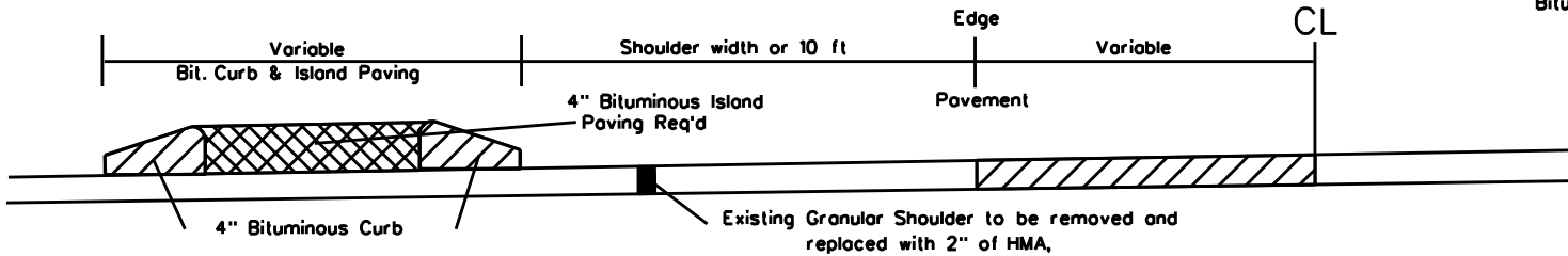
Typical Section of Bit. Curb & Bit. Island Placement on Existing Non-Paved Areas
