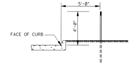
DELINEATOR MOUNTING ON CURBED CROSSOVER
