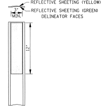
DETAIL OF TYPE II FLEXIBLE POST DELINEATOR
