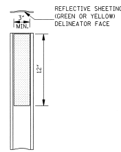
DETAIL OF TYPE I FLEXIBLE POST DELINEATOR
