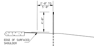
DELINEATOR MOUNTING ON CROSSOVER WITH USABLE SHOULDER
