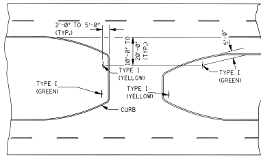
TYPICAL DELINEATION AT A CURBED CROSSOVER WITH A MEDIAN WIDTH OVER 40'-0"
