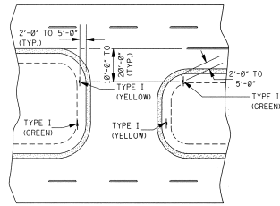
TYPICAL DELINEATION AT A CROSSOVER WITH USABLE SHOULDERS AND A MEDIAN WIDTH OVER 40'-0"
