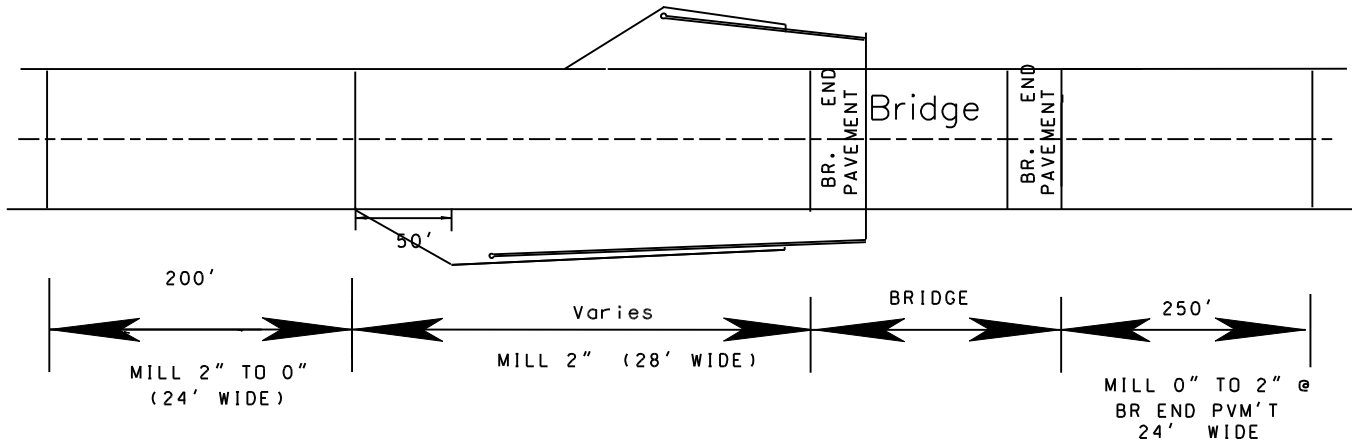
RIGHT LANE BRIDGES ----- NORTH BOUND
