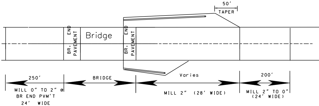
LEFT LANE BRIDGES ----- SOUTH BOUND
