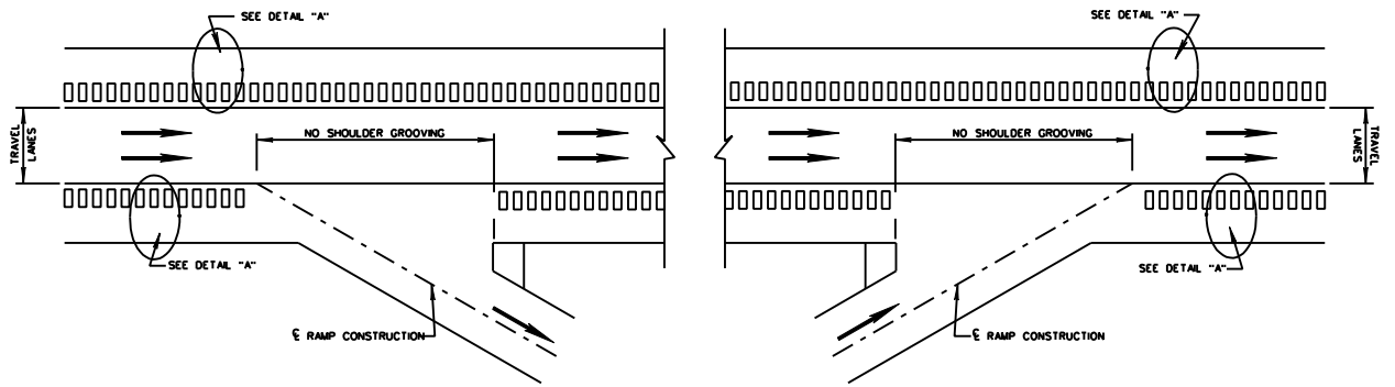
NOT TO SCALE DETAILS OF RUMBLE STRIPS (GROUND-IN)
