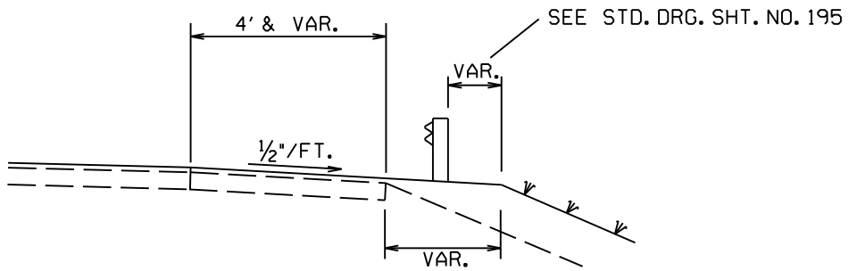
SECTION "A-A" BOTH SIDES
