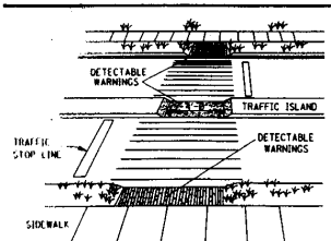
TRAFFIC ISLAND CUTAWAY NOTE: PASSAGE THROUGH TRAFFIC ISLAND SHALL BE FLUSH WITH ROADWAY.
