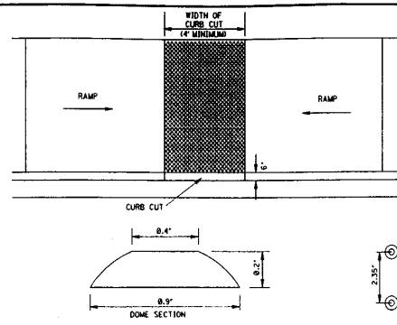
DETECTABLE WARNINGS (TRUNCATED DOMES) FOR BLIND & LOW VISION PEDESTRIANS
