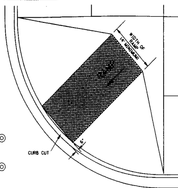
DETECTABLE WARNINGS (TRUNCATED DOMES) FOR BLIND & LOW VISION PEDESTRIANS
