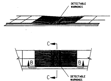
TYPE IV (TANGENT)
