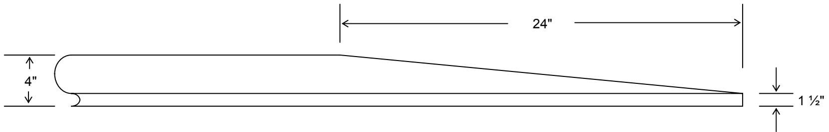
Bituminous Curb Terminus
