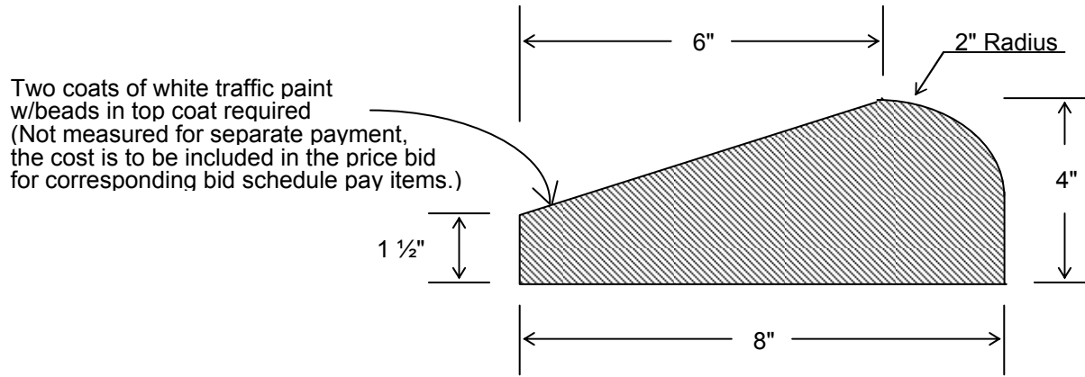
Bituminous Curb Cross Section
