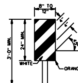
VERTICAL PANEL
