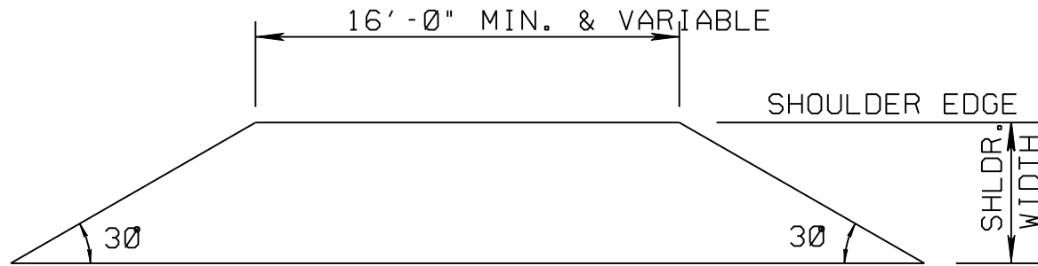
DETAIL OF PAVED APRON
