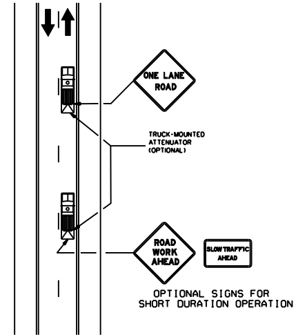
MOBILE OPERATIONS ON TWO-LANE ROAD
