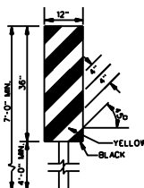
TYPE 3 OBJECT MARKER (OM-3R)
