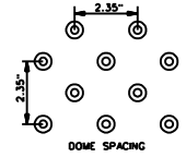
DETECTABLE WARNINGS (TRUNCATED DOMES) FOR BLIND & LOW VISION PEDESTRIANS
