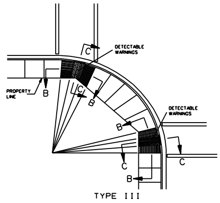
DETECTABLE WARNINGS (TRUNCATED DOMES) FOR BLIND & LOW VISION PEDESTRIANS
