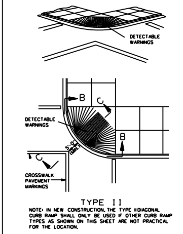
DETECTABLE WARNINGS (TRUNCATED DOMES) FOR BLIND & LOW VISION PEDESTRIANS
