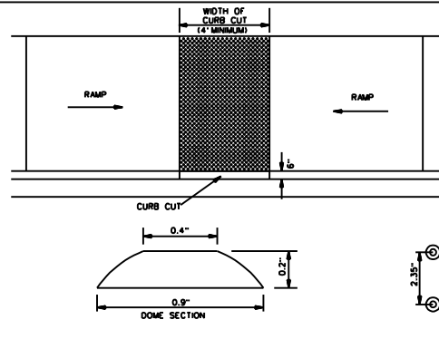
DETECTABLE WARNINGS (TRUNCATED DOMES) FOR BLIND & LOW VISION PEDESTRIANS
