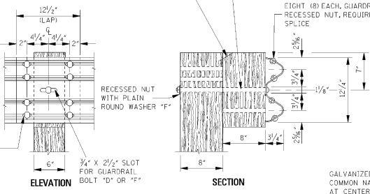
GUARDRAIL SPLICE DETAIL
