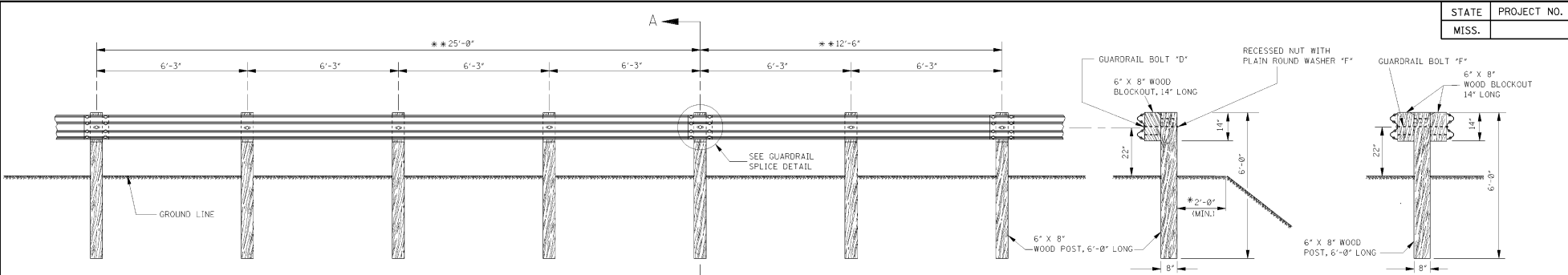
ELEVATION FROM \zeta ROADWAY ** NOTE: OPTIONAL BEAM LENGTHS.
