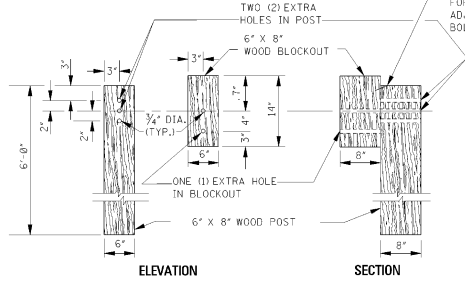
DETAILS OF ADJUSTABLE HEIGHT BLOCKOUT ASSEMBLY
