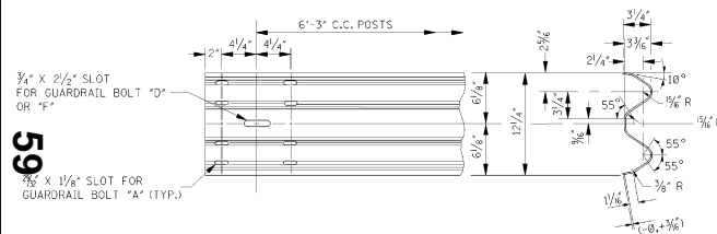
TYPICAL GUARDRAIL SECTION
