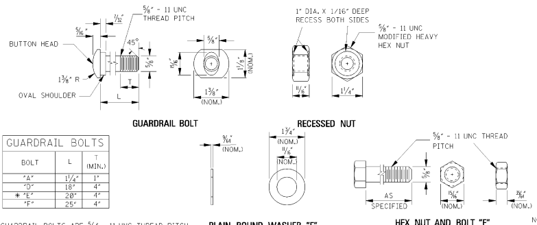
FASTENER DETAILS
