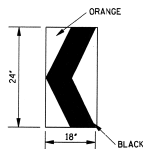
CHEVRON SIGN DETAIL
