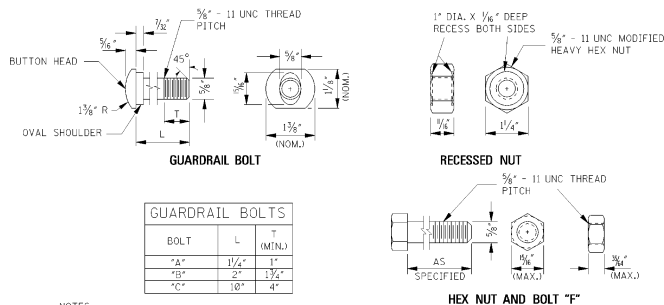
FASTENER DETAILS
