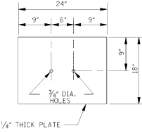
SOIL PLATE
