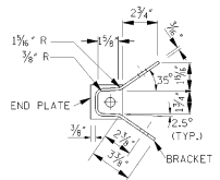
BRACKET
