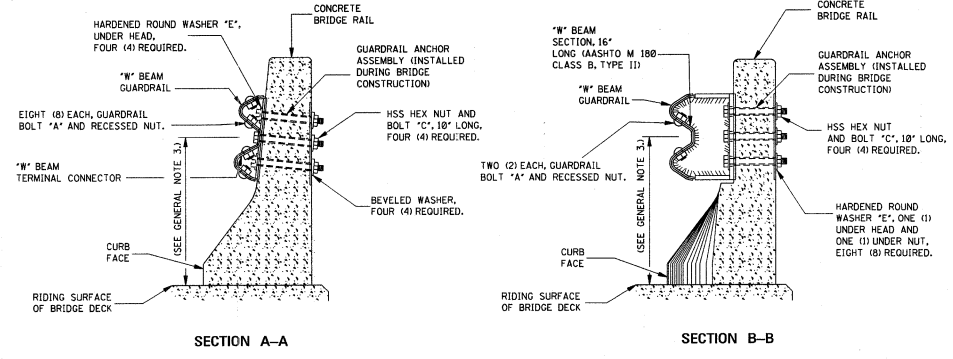
FACE ELEVATION SECTION GUARDRAIL CONNECTION DETAILS
