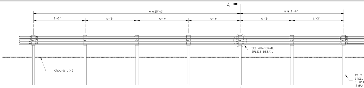
ELEVATION FROM C ROADWAY
