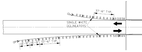
BRIDGE APPROACH INSTALLATION (TWO-WAY TRAFFIC)
