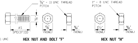
HEX NUT AND BOLT "F"
