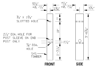
TERMINAL POST
