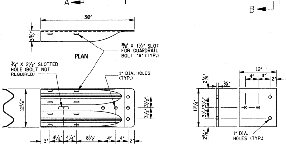
"W" BEAM TERMINAL CONNECTOR NOTE: THE "W" BEAM TERMINAL CONNECTOR IS USED WITH THE TYPE "G" MODIFIED BRIDGE END SECTION. THE CROSS-SECTIONAL DIMENSIONS OF THIS PART ARE IDENTICAL TO THE STANDARD "W" BEAM SECTION (AASHTO M 180 CLASS B, TYPE II). DETAIL OF PLATE "Y"
