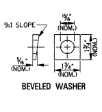
BEVELED WASHER
