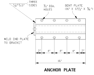
ANCHOR PLATE
