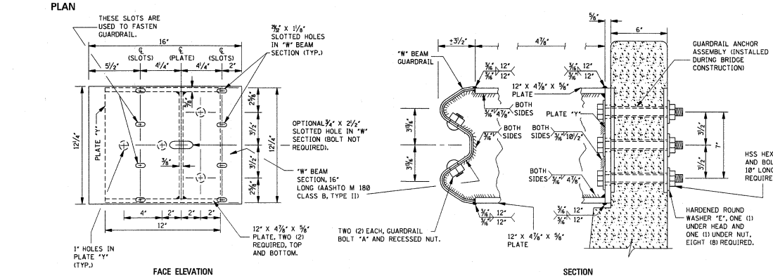
FACE ELEVATION SECTION GUARDRAIL CONNECTION DETAILS
