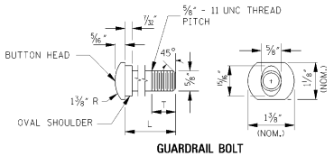
GUARDRAIL BOLT
