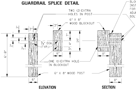
DETAILS OF ADJUSTABLE HEIGHT BLOCKOUT ASSEMBLY
