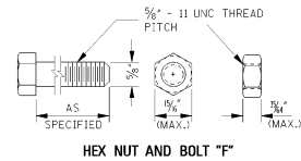
HEX NUT AND BOLT "F"
