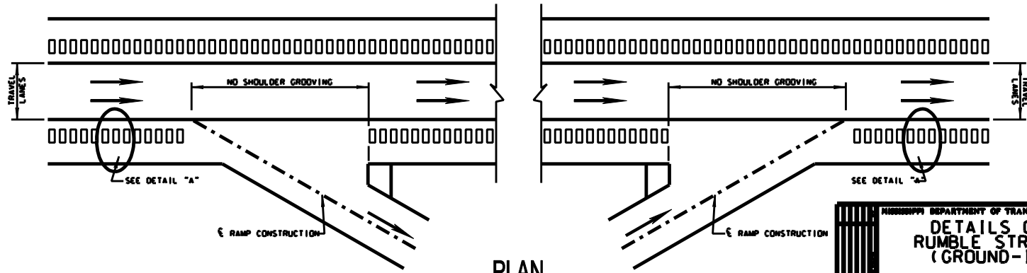
PLAN
