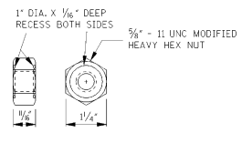
RECESSED NUT
