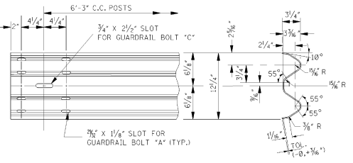
TYPICAL GUARDRAIL SECTION
