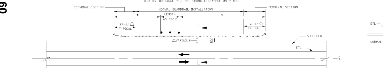
TYPICAL INSTALLATION FOR ROADSIDE OBSTACLE ON SIDE SLOPE 10:1 OR FLATTER * NOTE: DISTANCE REQUIRED SHOWN ELSEWHERE ON PLANS.
