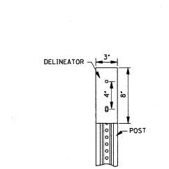
DETAIL OF SINGLE WHITE OR SINGLE YELLOW DELINEATOR
