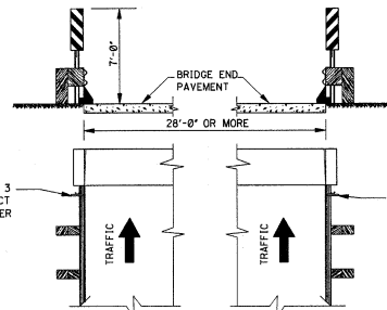
DETAIL OF TYPE 3 OBJECT MARKER INSTALLATION
