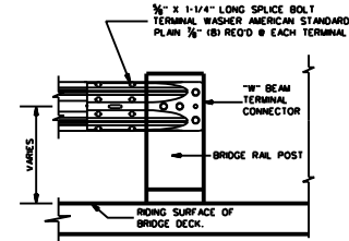
BRIDGE CONNECTOR END SECTION
