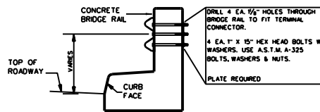
TERMINAL END SECTION
