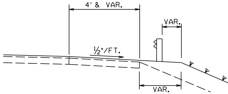
BOTH SIDES
