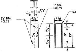
DETAIL OF BRIDGE END TERMINAL OFFSET BLOCK
