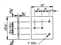
DETAIL OF PLATE "Y"
