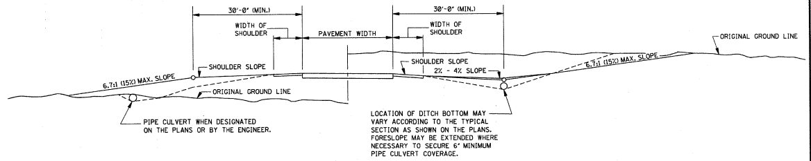
TYPICAL SECTION AT RAMP
