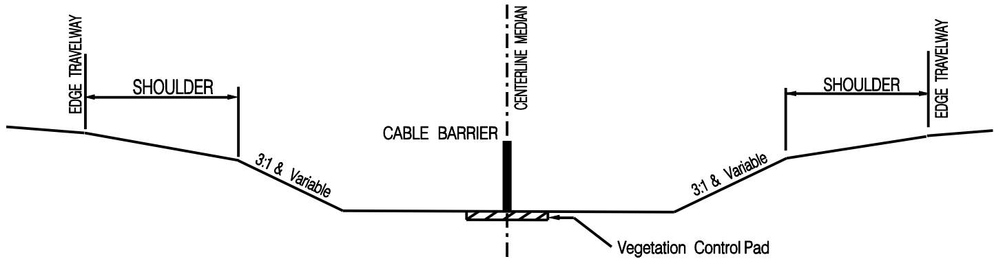
TYPICAL SECTION
