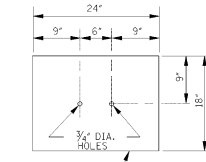
SOIL PLATE
