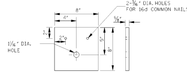
BEARING PLATE
