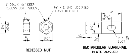
RECESSED NUT
