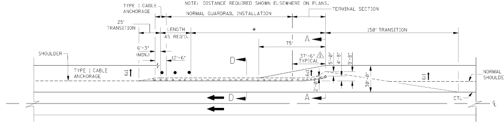
TYPICAL INSTALLATION FOR ROADSIDE OBSTACLE ON SIDE SLOPE STEEPER THAN 10:1
