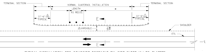
TYPICAL INSTALLATION FOR ROADSIDE OBSTACLE ON SIDE SLOPE 10:1 OR FLATTER *NOTE: DISTANCE REQUIRED SHOWN ELSEWHERE ON PLANS.
