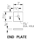
END PLATE
