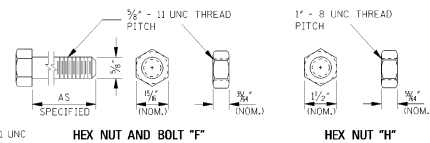
HEX NUT AND BOLT "F"
