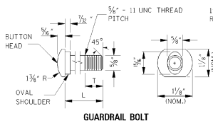
GUARDRAIL BOLT
