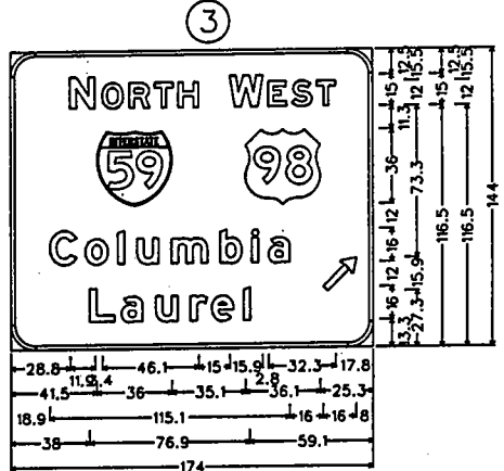
12.0" Radius, 2.0" Border, White on Green; [NORTH] E Mod; [WEST] E Mod; [Columbia] E Mod; [Laurel] E Mod; Standard Arrow Custom 21.0" X 8.5" 45!;
