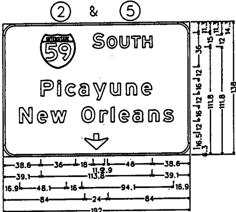
12.0" Radius, 2.0" Border, White on Green; [SOUTH] E Mod; [Picayune] E Mod; [New Orleans] E Mod; Down Arrow 16.0" 270!;
