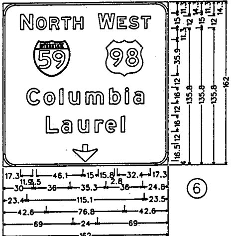
12.0" Radius, 2.0" Border, White on Green; [NORTH] E Mod; [WEST] E Mod; [Columbia] E Mod; [Laurel] E Mod; Down Arrow 16.0" 270!;
