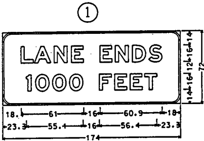
9.0" Radius, 1.5" Border, Black on Yellow; [LANE ENDS] E Mod; [1000 FEET] E Mod;
