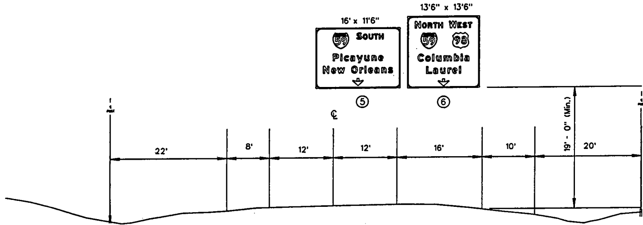
OVERHEAD SIGN ASSEMBLY "B" Located at the US 98 Westbound to I-59 Northbound Ramp Location to be staked by the Engineer.
