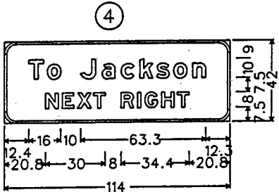
6.0" Radius, 1.3" Border, White on Green; [To Jackson] E Mod; [NEXT RIGHT] E Mod;
