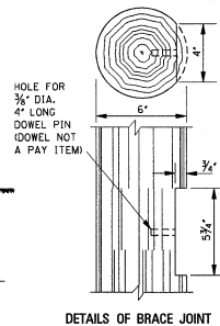
DETAILS OF BRACE JOINT
