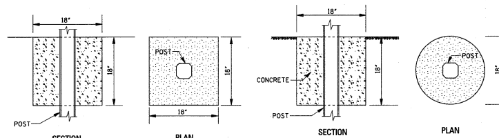
DETAIL OF POST ANCHOR
