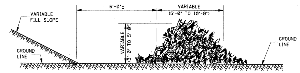
SIDE ELEVATION
