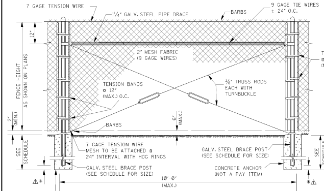
INTERMEDIATE BRACE BAY
