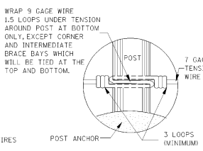
TENSION WIRE TIE DETAILS
