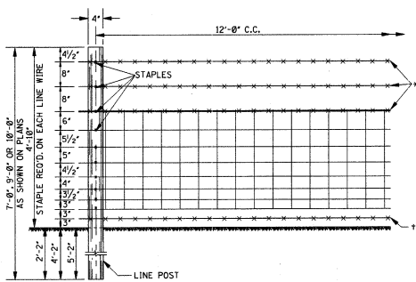
DETAILS OF LINE FENCE AND LINE POSTS
