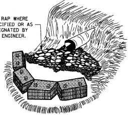
CULVERT
