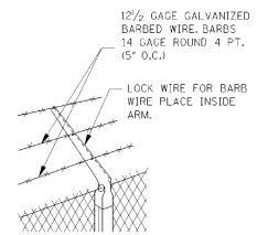
LINE POST TOP (VERTICAL ARMS WHEN DESIRED)
