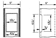
DETAIL OF BRACE JOINT
