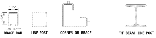
ALTERNATE TYPES OF BRACE RAIL, OR LINE, CORNER OR BRACE POST
