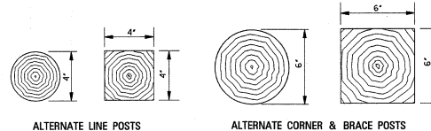
SECTIONS OF TIMBER POSTS
