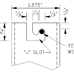
C-SECTION "J" SLOT DETAIL
