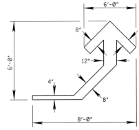
DETAIL OF TEMPORARY TURN ARROW
