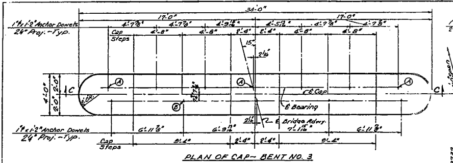
PLAN OF CAP-BENT NO. 3
