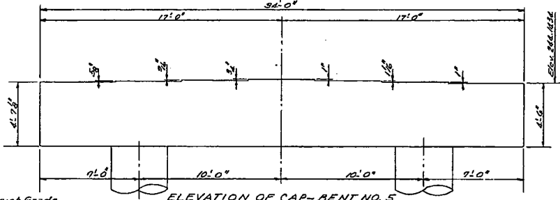
ELEVATION OF CAP-BENT NO. 5 Showing Cap Steps For 34'-0" Span
