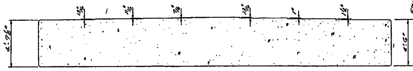
SECTION C-C Showing Cap Steps For 34'-0" Span.
