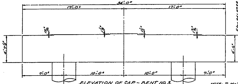
ELEVATION OF CAP-BENT NO. 3 Showing Cap Steps For 34'-0" Span
