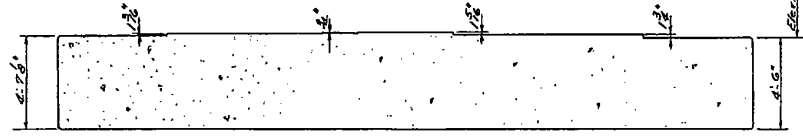
SECTION D-D Showing Cap Steps For 34'-0" Span
