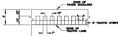
DETAIL "A"
