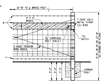
DETAIL OF CORNER BRACE
