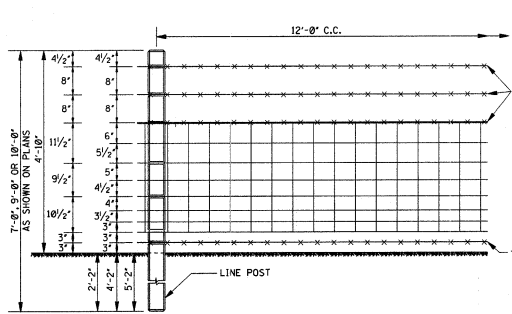
DETAILS OF LINE FENCE AND LINE POSTS
