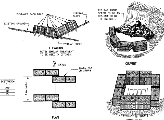
TEMPORARY EROSION CHECKS USING HAY OR STRAW BALES
