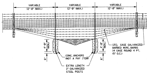
CROSSING TYPE III
