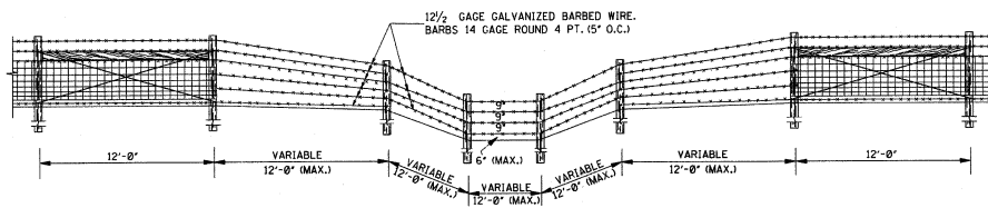
CROSSING TYPE I
