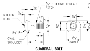
GUARDRAIL BOLTS
