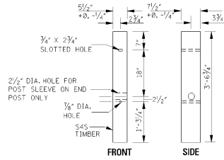
TERMINAL POST
