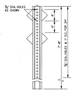
REAR VIEW OF DELINEATOR ASSEMBLY
