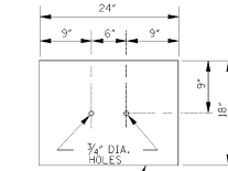
SOIL PLATE
