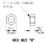
HEX NUT "H"
