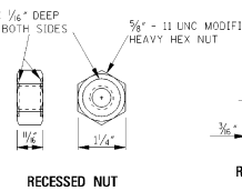
RECESSED NUT
