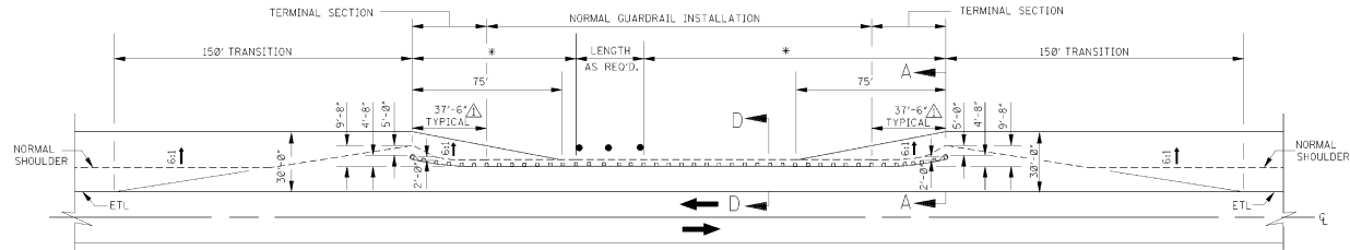
TYPICAL INSTALLATION FOR ROADSIDE OBSTACLE ON SIDE SLOPE STEEPER THAN 10:1 * NOTE: DISTANCE REQUIRED SHOWN ELSEWHERE ON PLANS.
