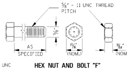
HEX NUT AND BOLT "F"
