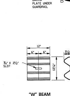
"W" BEAM BACKUP PLATE NOTE: THE "W" BEAM BACK-UP PLATE IS USED UNDER THE "W" BEAM RAIL SECTION WHERE INDICATED ON THIS SHEET. THE CROSS-SECTIONAL DIMENSIONS OF THIS PART ARE IDENTICAL TO THOSE OF THE STANDARD "W" BEAM RAIL SECTION.
