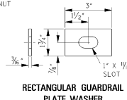
RECTANGULAR GUARDRAIL PLATE WASHER
