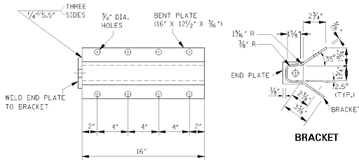
ANCHOR PLATE ASSEMBLY DETAILS
