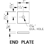
END PLATE
