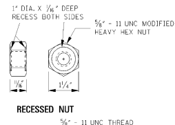
RECESSED NUT
