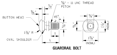
GUARDRAIL BOLT
