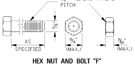
HEX NUT AND BOLT "F"
