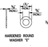
FASTENER DETAILS
