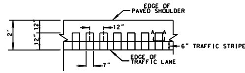
DETAIL "A"
