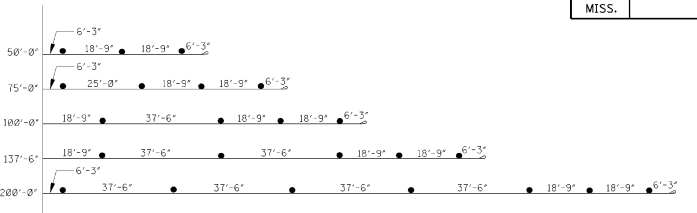
GRAPHIC SHOWING SPACINGS OF GUARDRAIL DELINEATORS AT SOME COMMONLY USED BRIDGE APPROACHES
