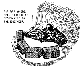
CULVERT
