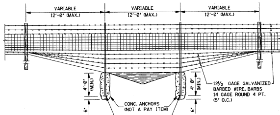
CROSSING TYPE III
