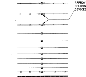
SPlicing DETAILS BETWEEN POSTS
