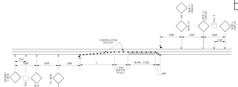
2 LANE - 2 WAY ROADWAY - LANE CLOSURE
