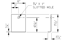
SHELF ANGLE BRACKET
