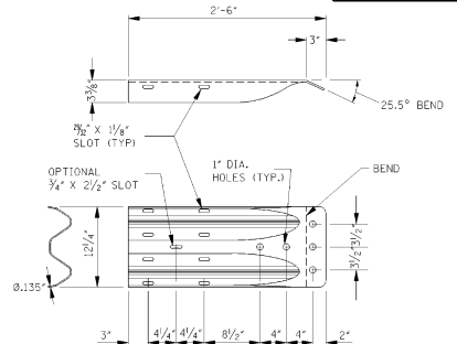
"W" BEAM TERMINAL CONNECTOR PLATE
