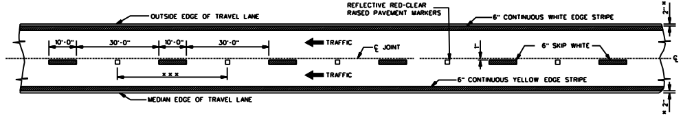
4-LANE WITH ONE-WAY TRAFFIC
