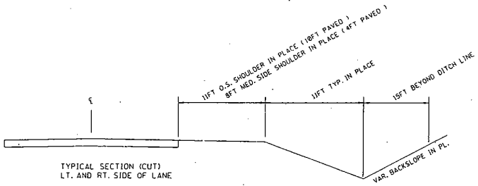
TYPICAL SECTIONS - ROADSIDE CLEAR ZONE REQ'D
