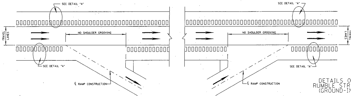
PLAN
