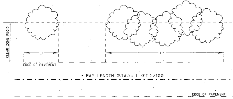
PAY DETAIL FOR RANDOM CLEARING
