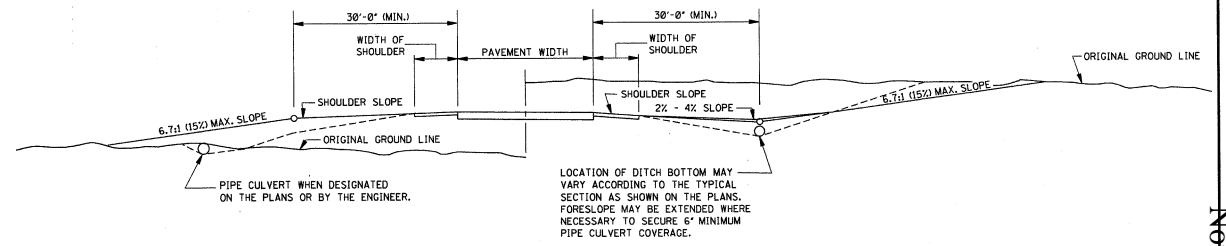
TYPICAL SECTION AT RAMP
