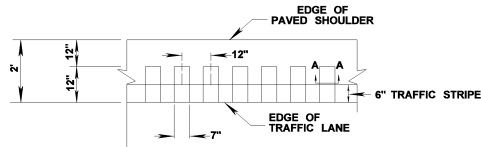
DETAIL "A"
