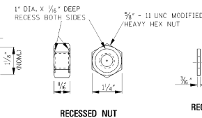
RECESSED NUT
