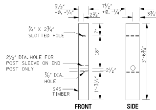
TERMINAL POST
