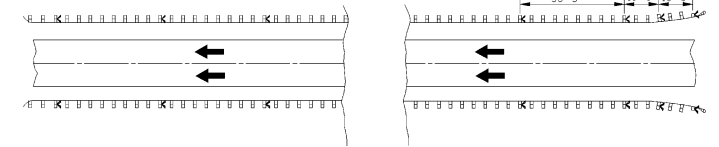
GRAPHIC SHOWING SPACINGS OF GUARDRAIL DELINEATORS AT SOME COMMONLY USED BRIDGE APPROACHES
