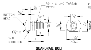
GUARDRAIL BOLT
