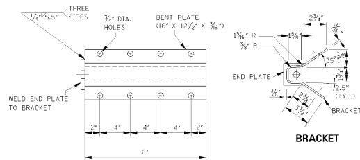
ANCHOR PLATE
