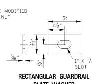
RECTANGULAR GUARDRAIL PLATE WASHER
