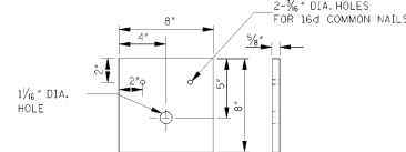
BEARING PLATE
