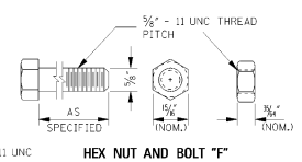
FASTENER DETAILS
