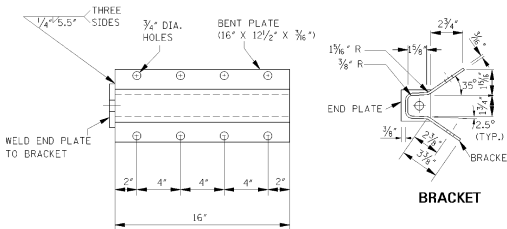
ANCHOR PLATE
