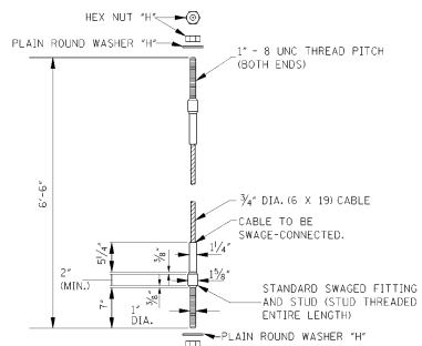
CABLE ANCHOR ASSEMBLY
