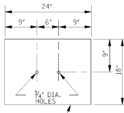
SOIL PLATE
