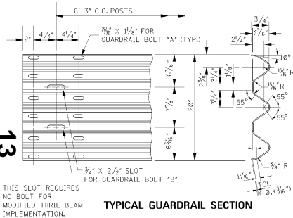
TYPICAL GUARDRAIL SECTION
