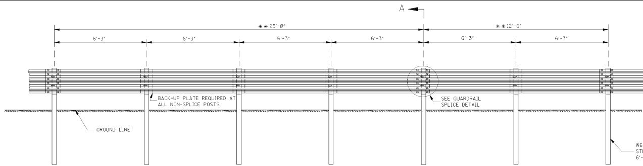
ELEVATION FROM \phi ROADWAY ** NOTE: OPTIONAL BEAM LENGTHS.
