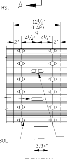
GUARDRAIL SPLICE DETAIL
