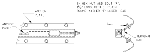
ANCHOR PLATE ASSEMBLY DETAILS
