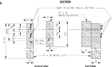
DETAILS OF ADJUSTABLE HEIGHT BLOCKOUT ASSEMBLY
