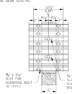
ELEVATION FROM Q ROADWAY **NOTE: OPTIONAL BEAM LENGTHS.
