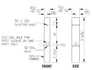
TERMINAL POST
