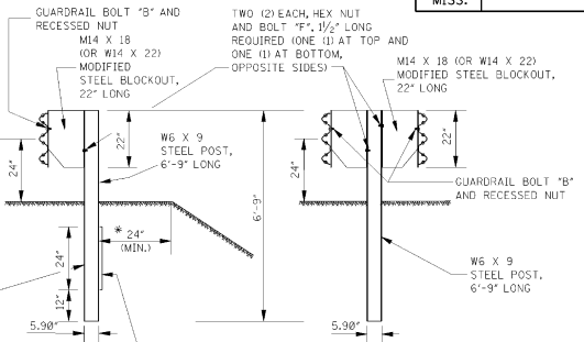
SINGLE-FACED BARRIER DOUBLE-FACED BARRIER SECTION A-A
