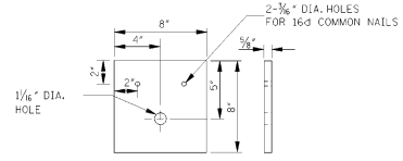
BEARING PLATE
