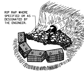
CULVERT
