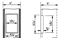
DETAIL OF BRACE JOINT
