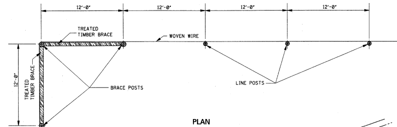
PLAN
