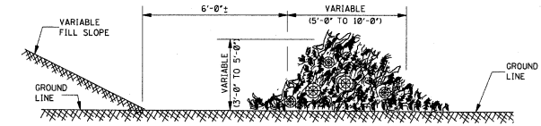
SIDE ELEVATION
