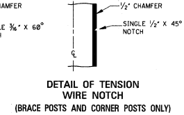
DETAIL OF TIE NOTCH (ALL POSTS)
