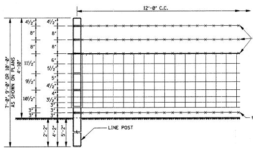
DETAILS OF LINE FENCE AND LINE POSTS
