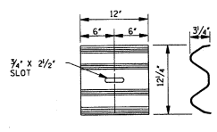
"W" BEAM BACKUP PLATE NOTE: THE "W" BEAM BACK-UP PLATE IS USED UNDER THE "W" BEAM RAIL SECTION WHERE INDICATED ON THIS SHEET. THE CROSS-SECTIONAL DIMENSIONS OF THIS PART ARE IDENTICAL TO THOSE OF THE STANDARD "W" BEAM RAIL SECTION.
