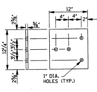
DETAIL OF PLATE "Y"
