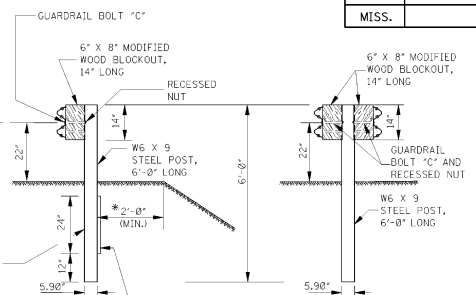
OPTIONAL: 24" X 12" STEEL SOIL BEARING PLATE, 1/4" THICK, WELDED TO POST WHERE SPECIFIED ON PLANS. WELD TOP, BOTTOM AND THREE 3" WELDS ON EACH SIDE.
