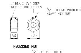
RECESSED NUT
