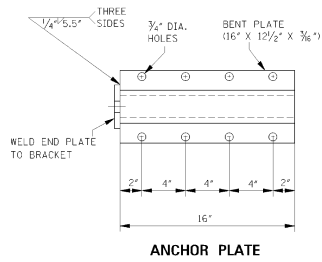
ANCHOR PLATE ASSEMBLY DETAILS
