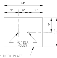
SOIL PLATE
