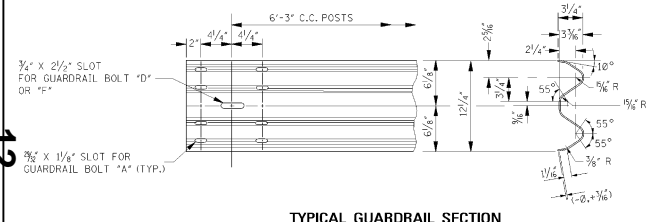
TYPICAL GUARDRAIL SECTION
