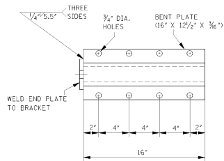
ANCHOR PLATE
