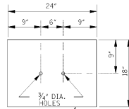
SOIL PLATE
