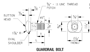
GUARDRAIL BOLT
