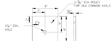
BEARING PLATE
