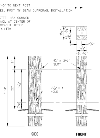
WOOD TIMBER POST NOTE: TERMINAL POST SHALL BE MADE OF S4S TIMBER WITH STRESS GRADE OF 1200 LB/IN 2 .
