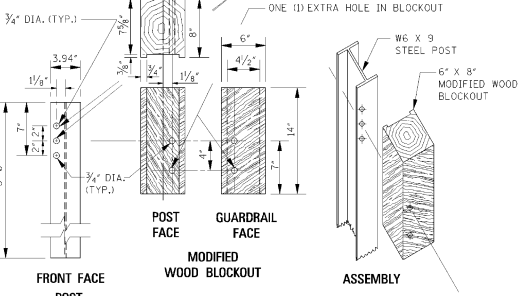
DETAILS OF ADJUSTABLE HEIGHT BLOCKOUT ASSEMBLY
