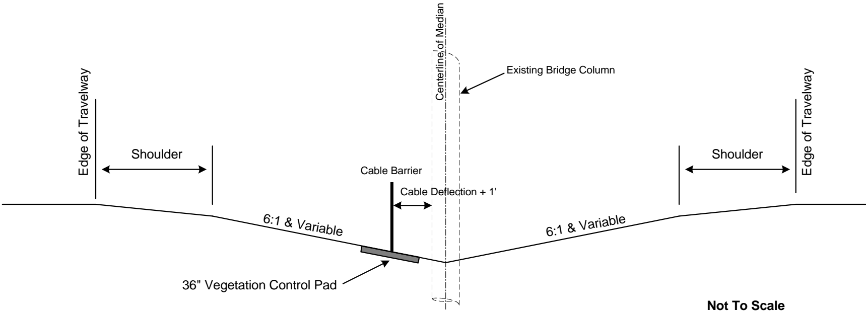
Typical Cable Barrier Detail at Bridge Column
