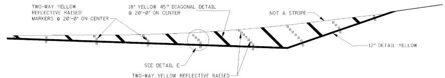
DETAIL B
