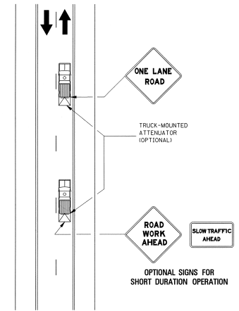
MOBILE OPERATIONS ON TWO-LANE ROAD
