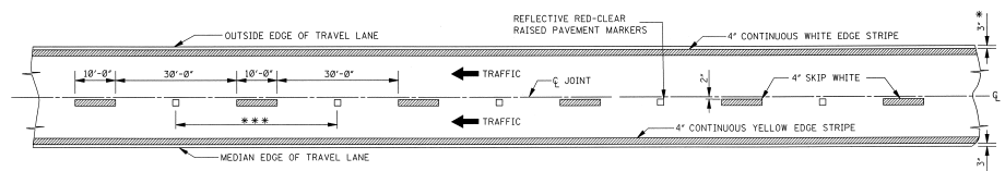
4-LANE WITH ONE-WAY TRAFFIC
