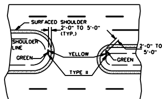
TYPICAL DELINEATION AT A CROSSOVER WITH USABLE SHOULDERS AND A MEDIAN WIDTH OF 40'-0" OR LESS
