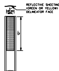
DETAIL OF TYPE I FLEXIBLE POST DELINEATOR
