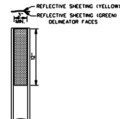
DETAIL OF TYPE II FLEXIBLE POST DELINEATOR
