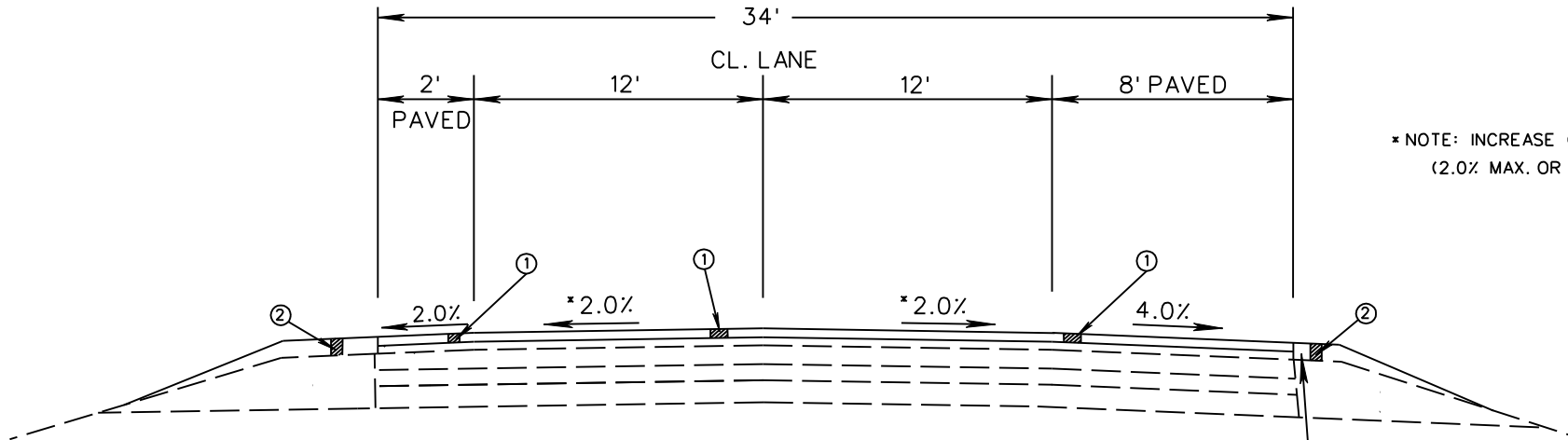
TYPICAL SECTION LT. & RT LANES (IN THE DIRECTION OF TRAFFIC)
