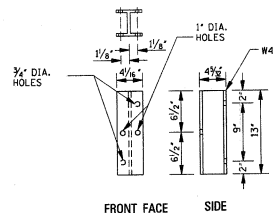
DETAIL OF BRIDGE END TERMINAL OFFSET BLOCK
