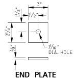
END PLATE
