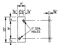
DETAIL OF PLATE "B"
