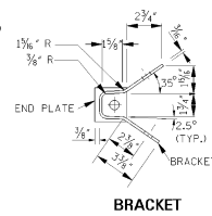
BRACKET
