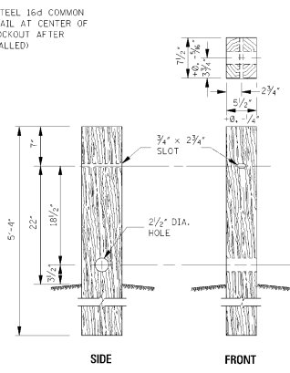
WOOD TIMBER POST NOTE: TERMINAL POST SHALL BE MADE OF S4S TIMBER WITH STRESS GRADE OF 1200 LB/IN 2 .
