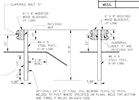
SINGLE-FACED BARRIER DOUBLE-FACED BARRIER SECTION A-A * NOTE: UNLESS SPECIFIED OTHERWISE ON THE PLANS.
