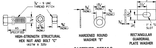
FASTENER DETAILS
