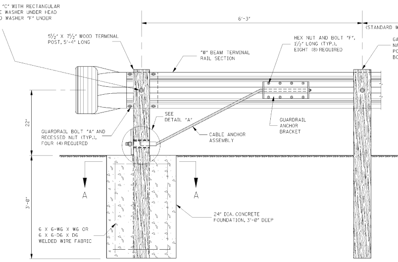
ELEVATION FROM BEHIND GUARDRAIL NOTE: ANCHOR CABLE SHALL BE TAUT.
