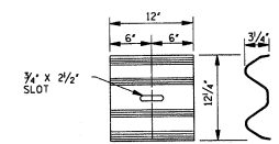
"W" BEAM BACKUP PLATE
