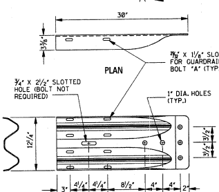
"W" BEAM TERMINAL CONNECTOR NOTE: THE "W" BEAM TERMINAL CONNECTOR IS USED WITH THE TYPE "D" MODIFIED BRIDGE END SECTION. THE CROSS-SECTIONAL DIMENSIONS OF THIS PART ARE IDENTICAL TO THE STANDARD "W" BEAM SECTION (AASHTO M 188 CLASS B, TYPE III).
