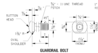
GUARDRAIL BOLTS
