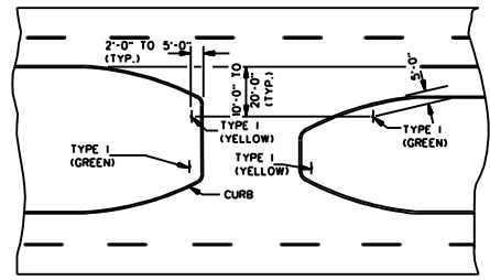
TYPICAL DELINEATION AT A CROSSOVER WITH USABLE SHOULDERS AND A MEDIAN WIDTH OVER 40'-0"
