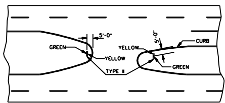
TYPICAL DELINEATION AT A CROSSOVER WITH USABLE SHOULDERS AND A MEDIAN WIDTH OF 40'-0" OR LESS
