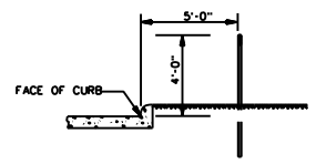
DELINEATOR MOUNTING ON CURBED CROSSOVER
