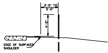
DELINEATOR MOUNTING ON CROSSOVER WITH USABLE SHOULDER
