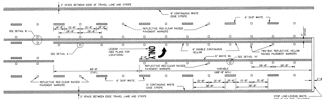
TYPICAL STRIPING AND RAISED PAVEMENT MARKERS AT LEFT TURN LANES *NOTE: USE DETAIL STRIPING IF LENGTH \leq 150' AT THIS LOCATION, OTHERWISE USE CONTINUOUS STRIPING.
