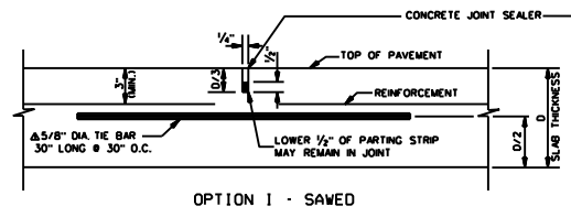
OPTION I - SAWED
