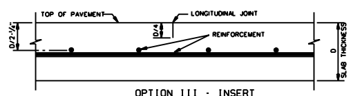
OPTION III - INSERT
