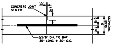
LONGITUDINAL CONSTRUCTION JOINT
