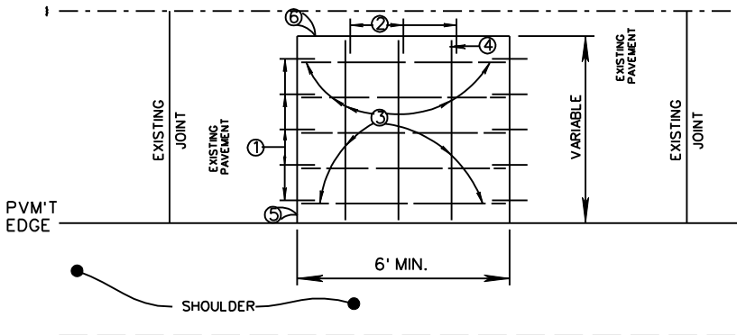
DETAIL OF TYPICAL FAILURE REPAIR
