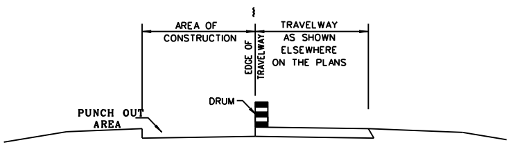
ELEVATION VIEW FOR DRUM
