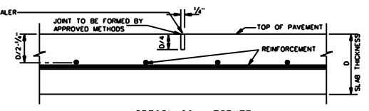
OPTION II - FORMED
