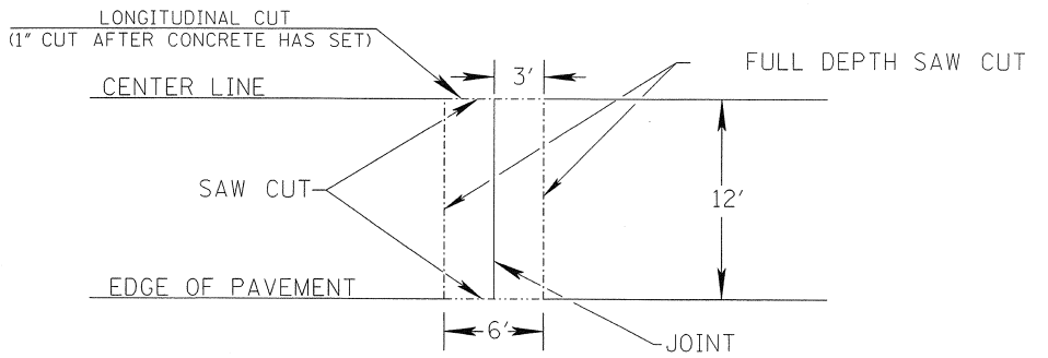
12' X 6' PUNCH OUT
