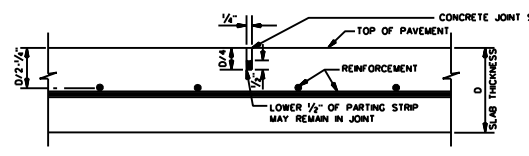
OPTION I - SAWED
