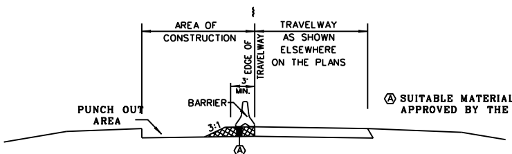
ELEVATION VIEW FOR POSITIVE BARRIER
