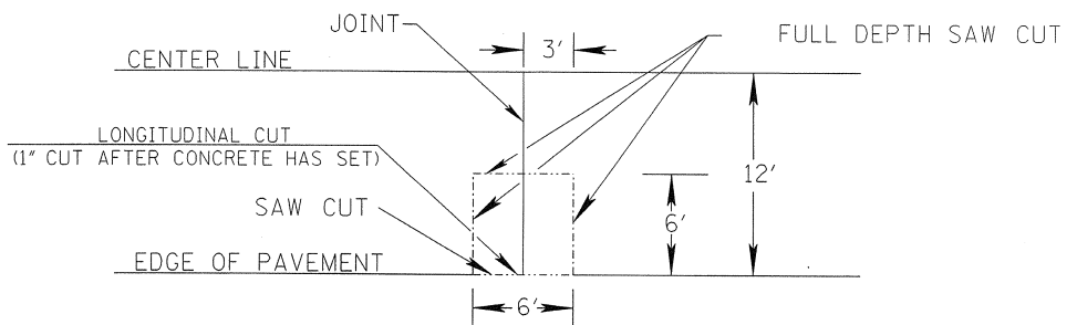
6' X 6' PUNCH OUT
