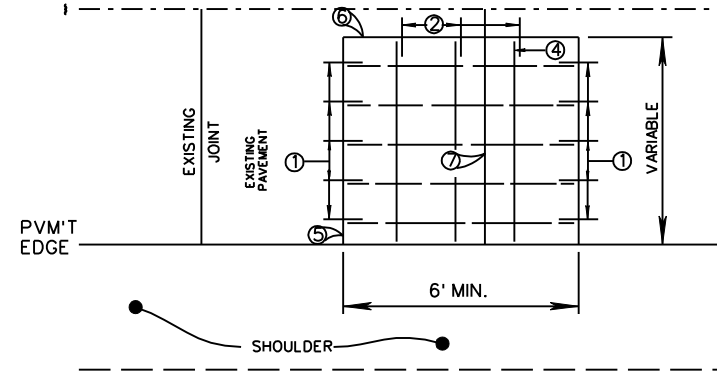
REPAIR OF FAILURE INCLUDING EXPANSION JOINT
