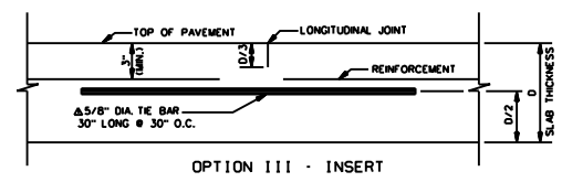
OPTION III - INSERT
