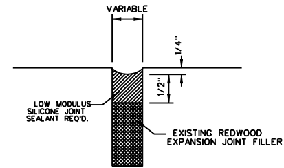
DETAIL FOR SEALING EXPANSION JOINTS
