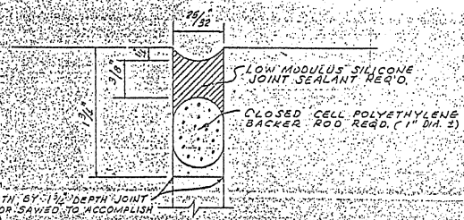
DETAIL FOR SEALING TRANSVERSE EXPANSION JOINTS (TYPE S-1) (NEW CONSTRUCTION)
