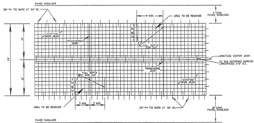
PLAN VIEW JOINT REPAIRS
