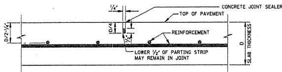
OPTION I - SAWed
