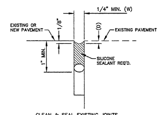
CLEAN & SEAL EXISTING JOINTS JOINT SEAL NO. 5
