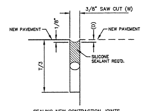
SEALING NEW CONSTRUCTION JOINTS JOINT SEAL NO. 4
