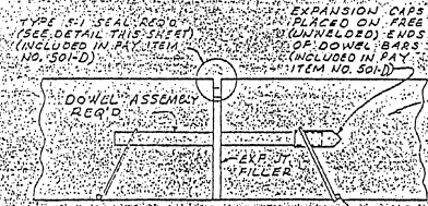
TYPE I (WITH DOWELS) (ALL NEW CONSTRUCTION) FOR DETAILS AND DIMENSIONS NOT SHOWN SEE SHEET NO. 04
