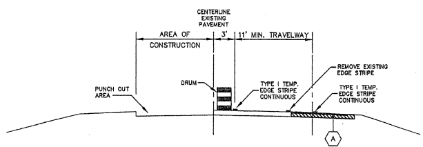
ELEVATION VIEW FOR DRUM
