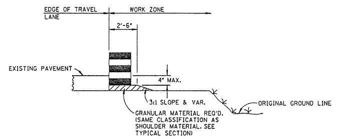
DETAIL OF DRUM PLACEMENT ON LOW SHOULDERS
