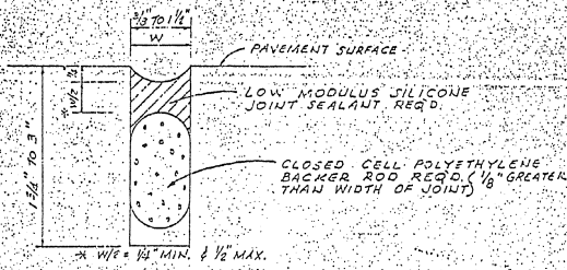
DETAIL FOR SEALING EXISTING TRANSVERSE JOINTS DOWELED OR UNDOWELED (TYPE S-4) (NOT RECONSTRUCTED OR OVERLAID) (PAY ITEM NO. 307-508-A)
