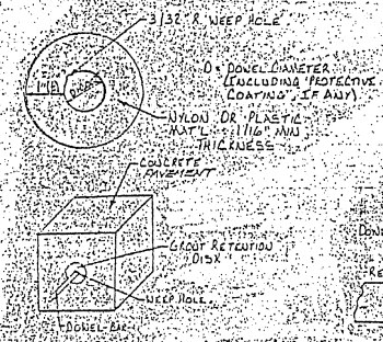
DETAIL OF ANCHORING MATERIAL RETENTION DISK FOR FULL DEPTH REPAIR DOWEL INSTALLATION
