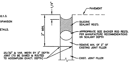
CLEAN & SEAL EXISTING EXPANSION JOINTS JOINT SEAL NO. 6 DETAIL OF EXPANSION JOINTS
