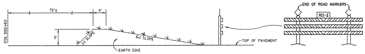
ROADWAY CLOSURE DETAIL (LONG-TERM)
