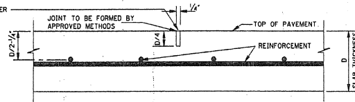
OPTION II - FORMED
