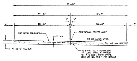
SECTION OF PORTLAND CEMENT CONCRETE PAVEMENT
