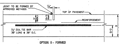
OPTION II - FORMED
