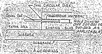
DOWEL ANCHORING
