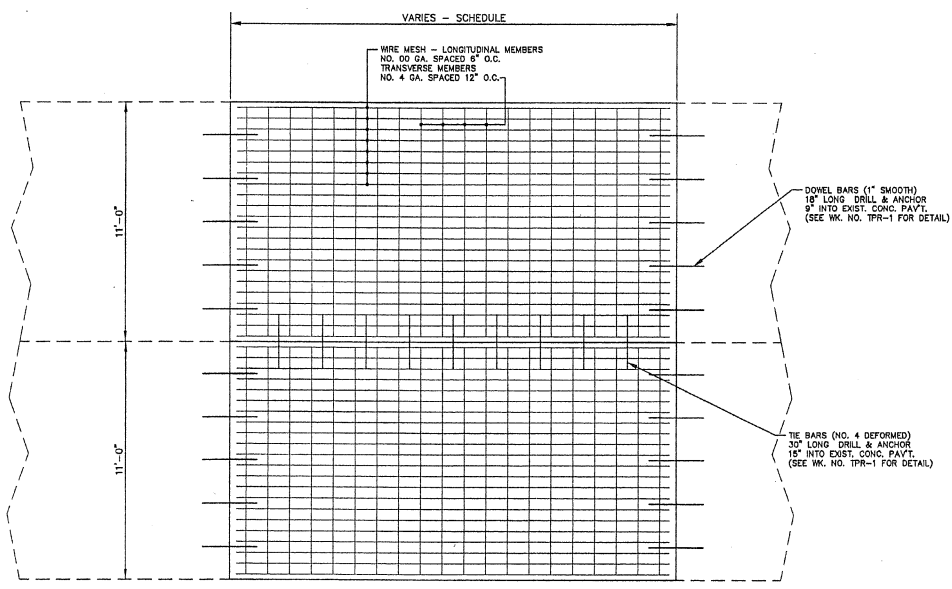
PLAN OF PORTLAND CEMENT CONCRETE PAVEMENT
