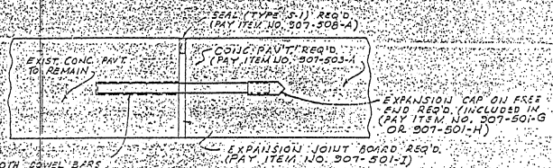
TYPE II (WITH DOWELS)
