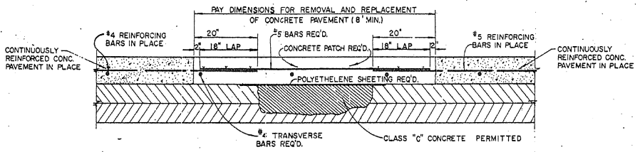
SECTIONAL VIEW (SHOWING REPLACED AREA)
