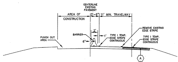
ELEVATION VIEW FOR POSITIVE BARRIER
