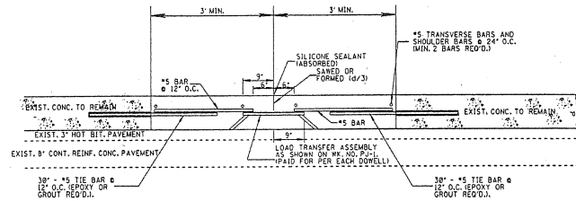
SECTIONAL VIEW OF REPLACED JOINT
