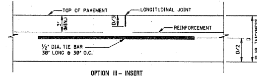
OPTION III - INSERT
