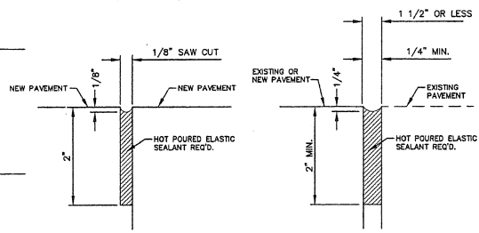
SEALING NEW CONSTRUCTION JOINTS JOINT SEAL NO. 1 CLEAN & SEAL EXISTING JOINTS JOINT SEAL NO. 2 DETAIL OF LONGITUDINAL JOINTS
