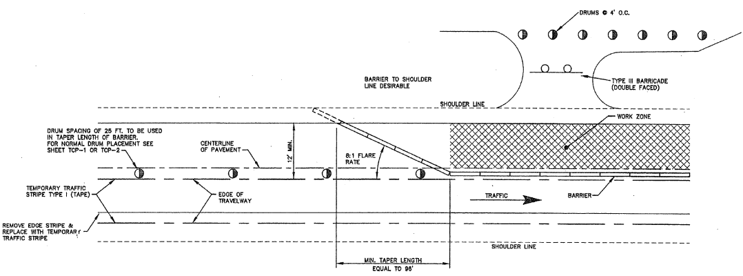
DETAIL OF TAPER FOR POSITIVE BARRIER IN WORK ZONE
