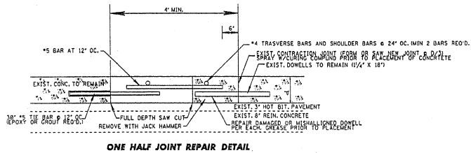
ONE HALF JOINT REPAIR DETAIL
