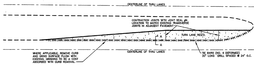
PLAN VIEW OF EXPANSION JOINTS AND DOWELS STA. 719+23.81 & 729+11.44 (4 TOTAL REQ'D.) SEE WK. NO. MDN-12 & MDN-13
