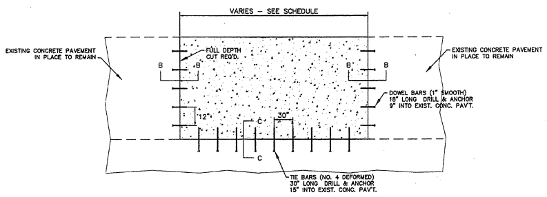
PLAN VIEW OF 8" JOINTED CONCRETE SLAB REPLACEMENT (SEE SDPD-1 FOR REINFORCEMENT REQUIREMENTS)
