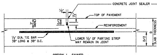
OPTION I - SAWed
