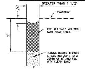
CLEAN & SEAL EXISTING JOINTS JOINT SEAL NO. 3
