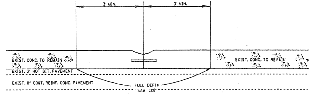
FULL JOINT REPAIR DETAIL
