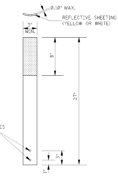
DETAIL OF FLEXIBLE GUARDRAIL DELINEATOR
