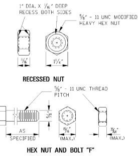
HEX NUT AND BOLT "F"
