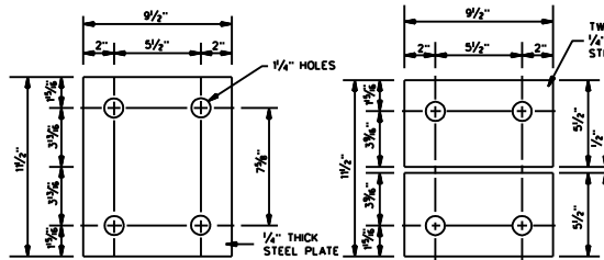
DETAIL OF PLATE "Z" CONCRETE BRIDGE RAIL (TYPE "A" & "C" BESS)
