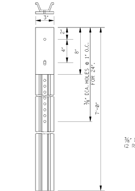
DETAIL OF SINGLE WHITE OR SINGLE YELLOW DELINEATOR
