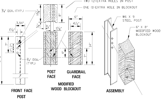
DETAILS OF ADJUSTABLE HEIGHT BLOCKOUT ASSEMBLY
