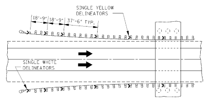
ROADSIDE OBSTACLE INSTALLATION—LENGTH 250' OR LESS (ONE-WAY TRAFFIC)
