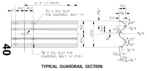
TYPICAL GUARDRAIL SECTION
