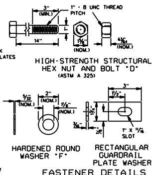
FASTENER DETAILS
