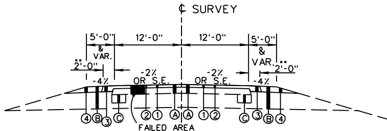
TYPICAL SECTION HWY. 27 STA. 10+00 TO STA. 625+20 (FROM HWY 18 JUST NORTH OF UTICA TO WARREN COUNTY LINE)
