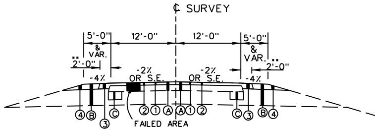
TYPICAL SECTION HWY. 27 B.O.P. STA. 0+48.30 TO STA. 601+52.19 (FROM COPIAH LINE TO HWY 18 AT UTICA)
