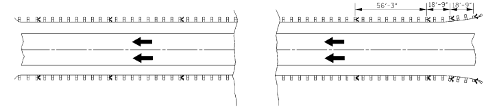
EMBANKMENT OR ROADSIDE OBSTACLE INSTALLATION—LENGTH GREATER THAN 250' (ONE-WAY TRAFFIC)
