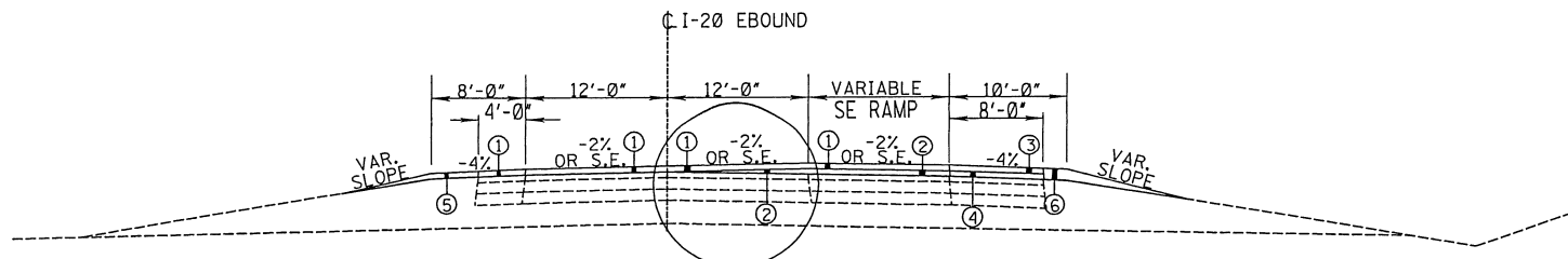
TYPICAL SECTION I-20 EBOUND B.O.P. STA. 1043+00 (+/-) TO STA. 1056+00 (+/-)
