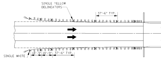
BRIDGE APPROACH INSTALLATION (ONE-WAY TRAFFIC)
